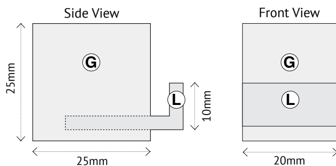
G + L Part Dimensions
