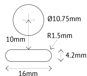
Back Panel Hole + Slot Dimensions
